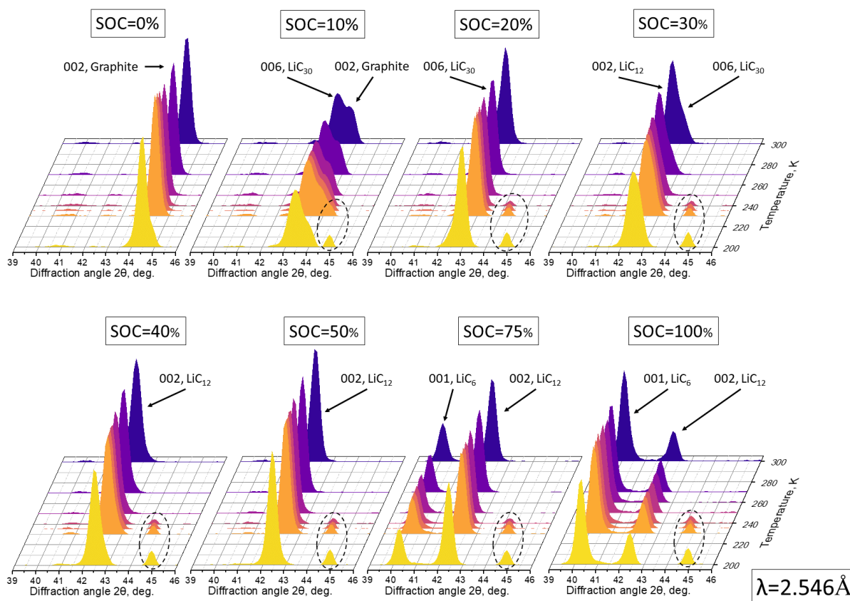
Figure 1. High-resolution neutron data collected from various SOC's showing reflection bunches of 002 reflection for graphite and \text{LiC}_{12} , 006 reflection for \text{LiC}_{30} and 001 reflection for \text{LiC}_6 with the electrolyte reflection appearing below 240 K. The origination of the electrolyte reflection and its evolution is marked by dashed ellipses.
